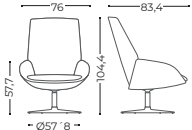
Aluminium round base Base redonda de aluminio
